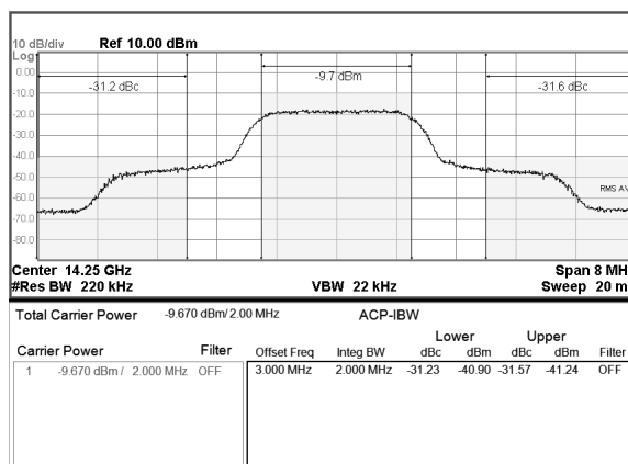
P_{OUT}=36\text{dBm} IDQ=2.45\text{A}
